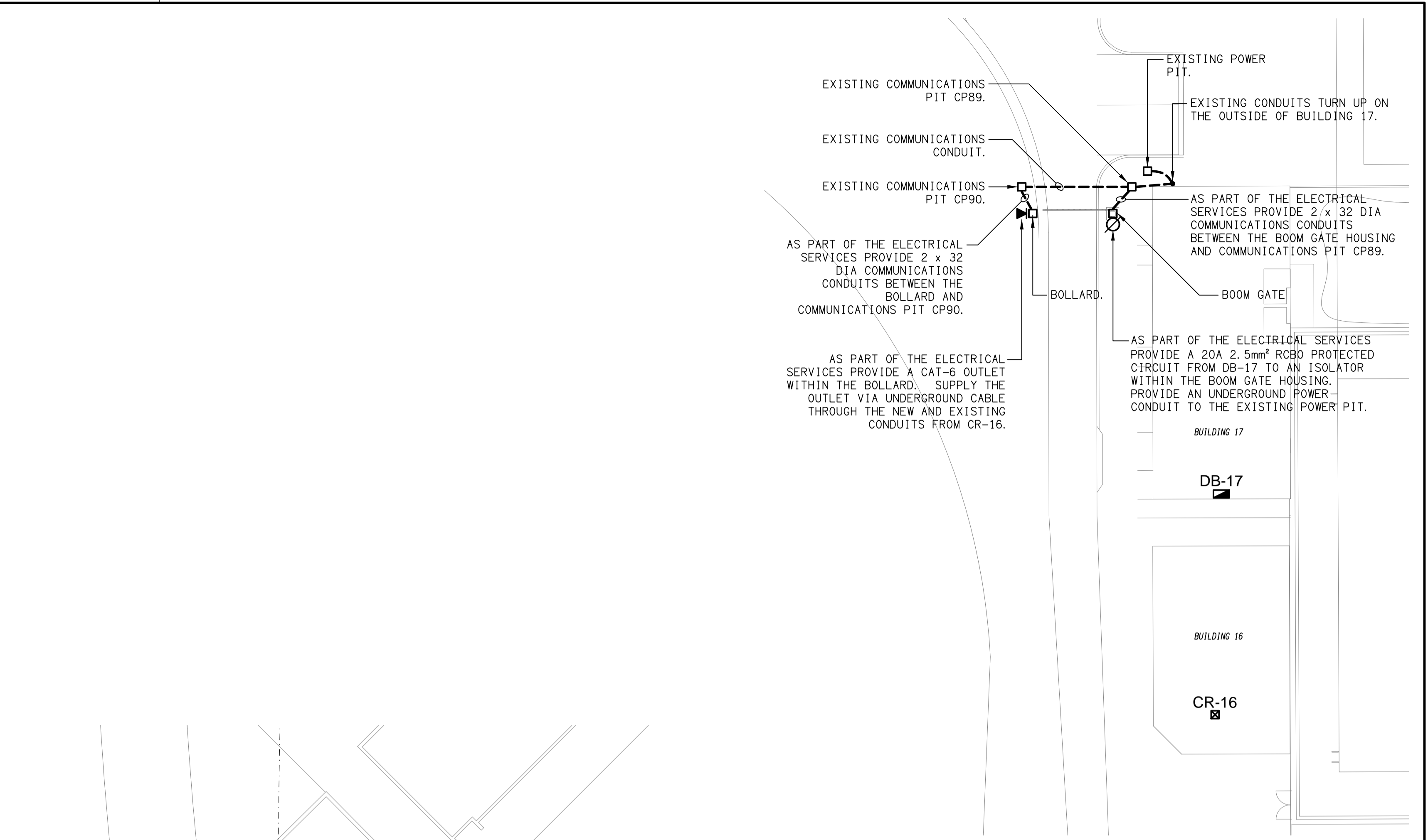
NORTH BOOM GATE DETAILED ELECTRICAL PLAN SCALE 1:200
